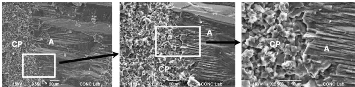
Figure 2.3 – Interface between aggregate particle and cement paste [55]
