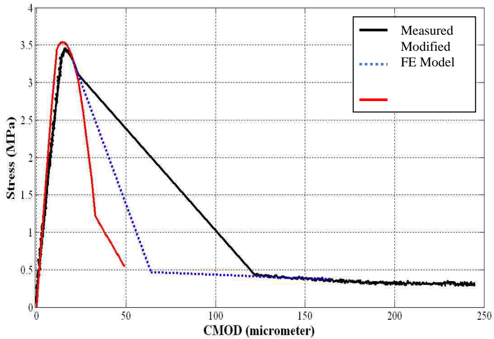
Figure 4.27 - Comparison of SCC3 experimental data, bilinear approximation, and model output
