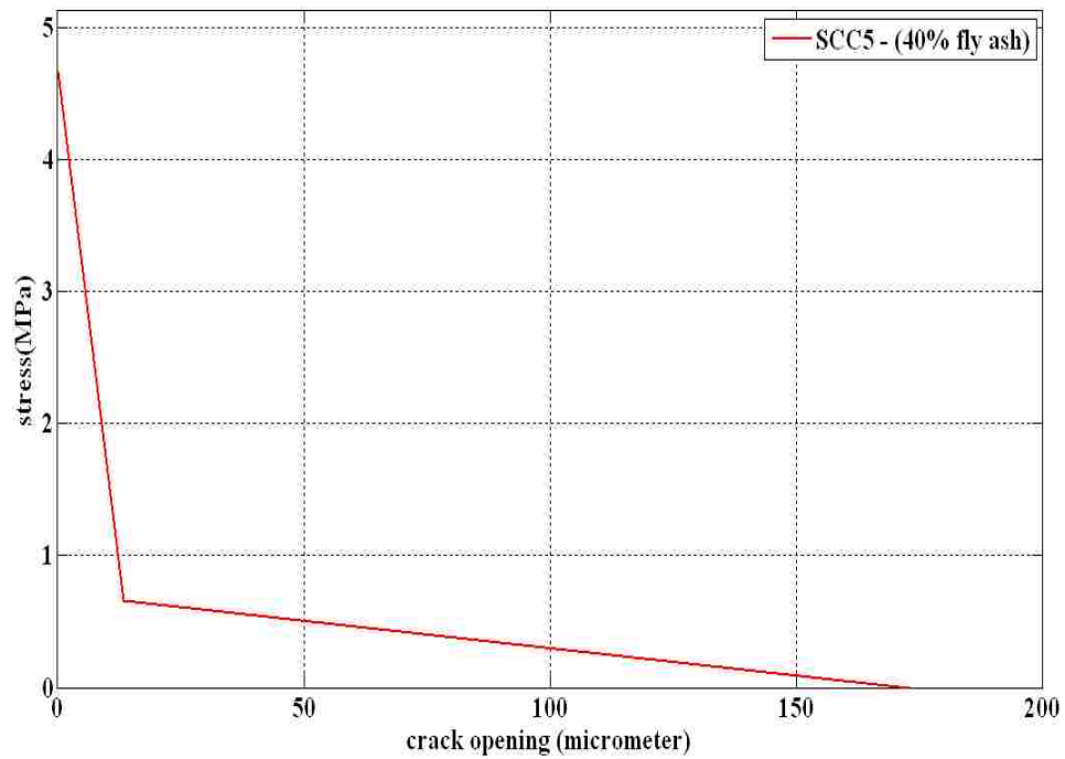
Figure 4.19 – Bilinear curve – SCC5
