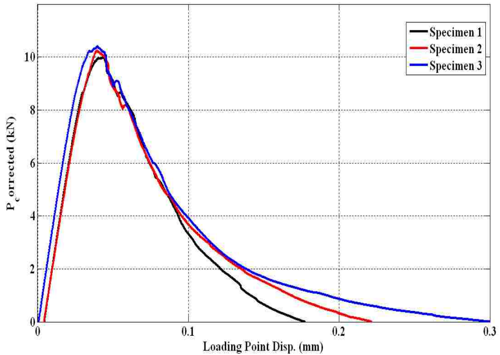
Figure 4.16 – Corrected load vs. displacement curve for SCC5
